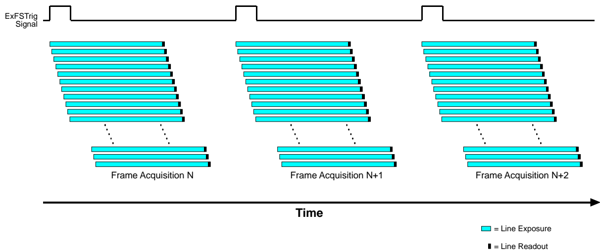
Fig. 68: Non-overlapped Acquisition
