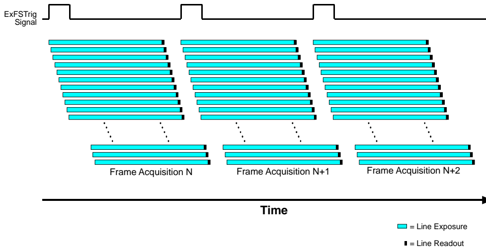
Fig. 69: Overlapped Exposure and Sensor Readout
