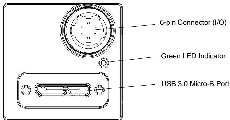
Fig. 37: Camera Connectors
