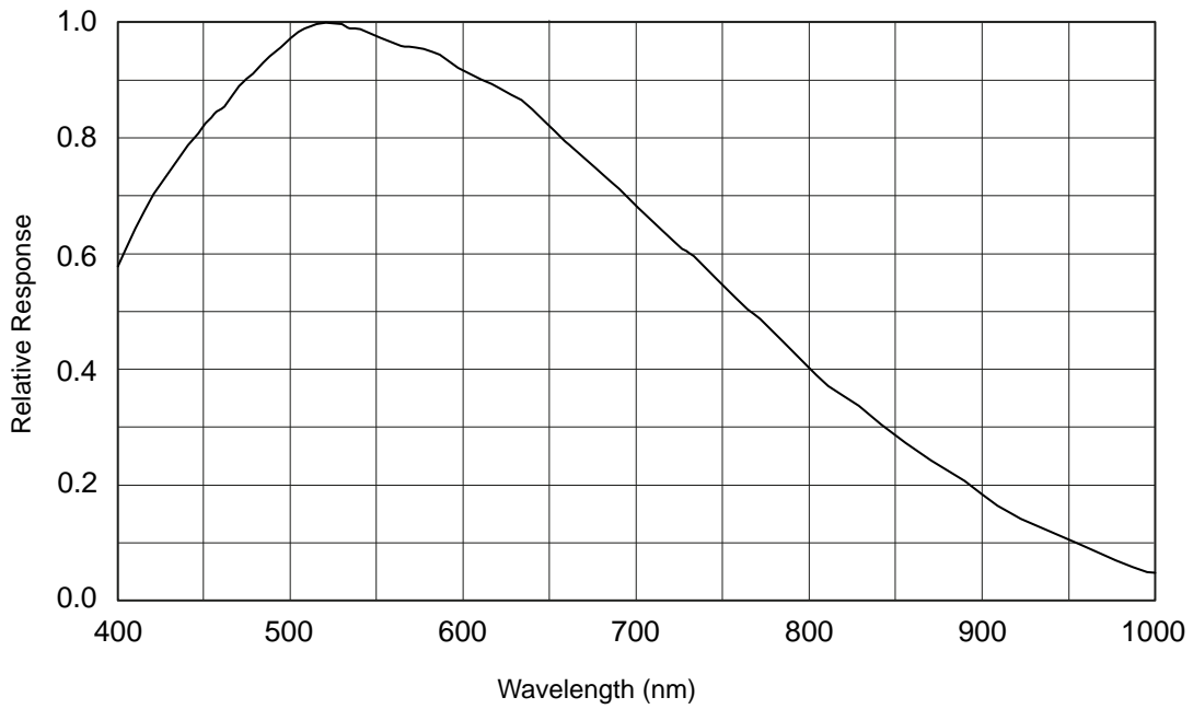
Fig. 7: acA1920-40um and acA1920-155um Spectral Response (From Sensor Data Sheet)
