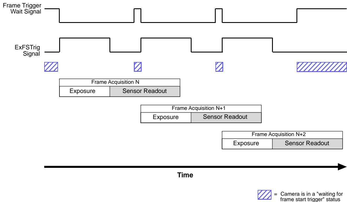
Fig. 75: Frame Trigger Wait Signal
