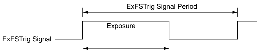
Fig. 57: Trigger Width Exposure with Rising Edge Triggering
