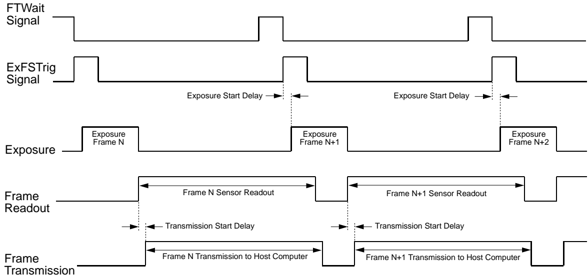
Fig. 79: Exposure Start Controlled with an ExFSTrig Signal
