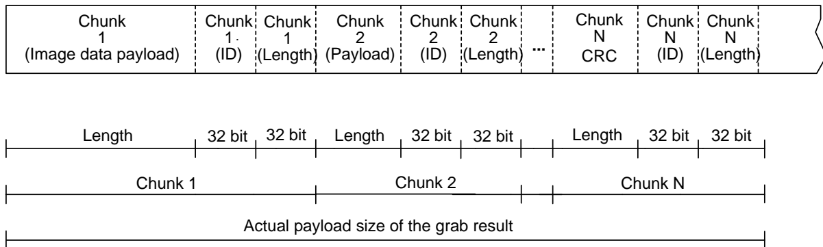
Fig. 116: Example of a Set of Chunks Related to One Image Acquisition
