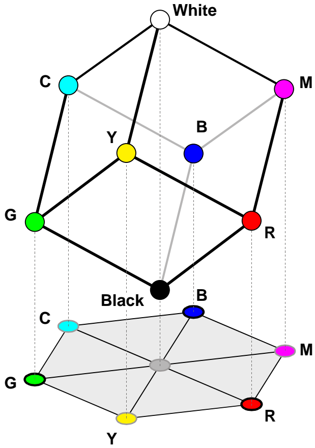
Fig. 107: RGB Color Cube With YCM Secondary Colors, Black, and White, Projected On a Plane
