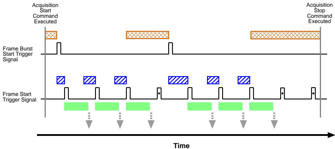
Fig. 53: Frame Burst Start and Frame Start Triggering
