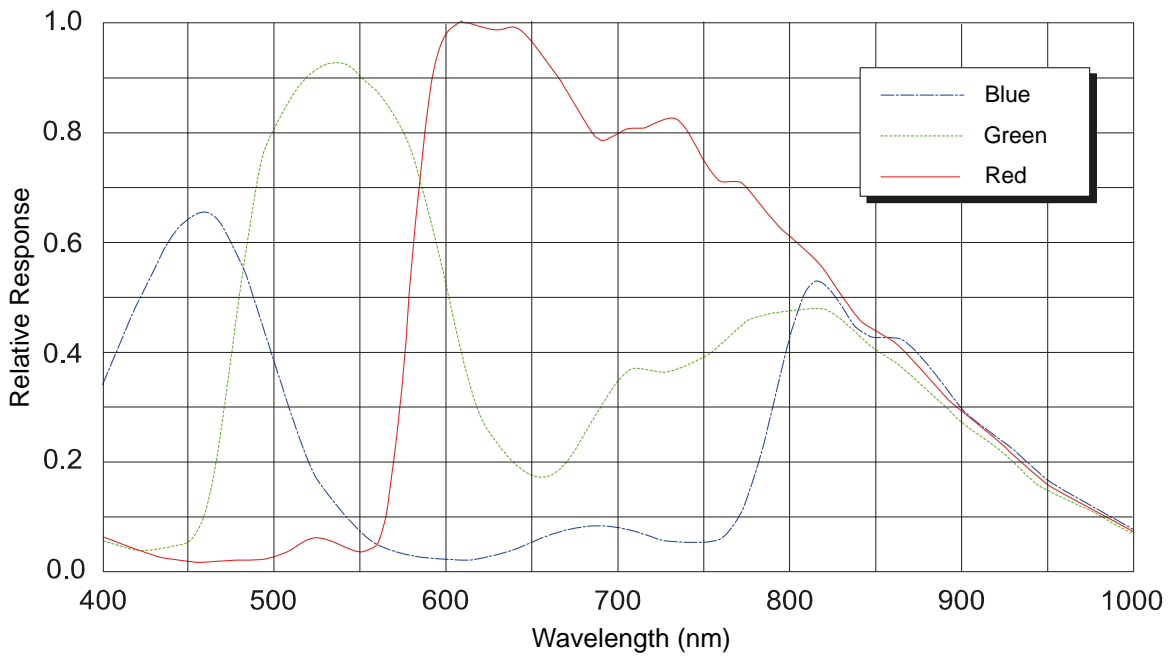
Fig. 21: acA2040-55uc, acA2040-120uc, acA2440-35uc, and acA2440-75uc (From Sensor Data Sheet)
