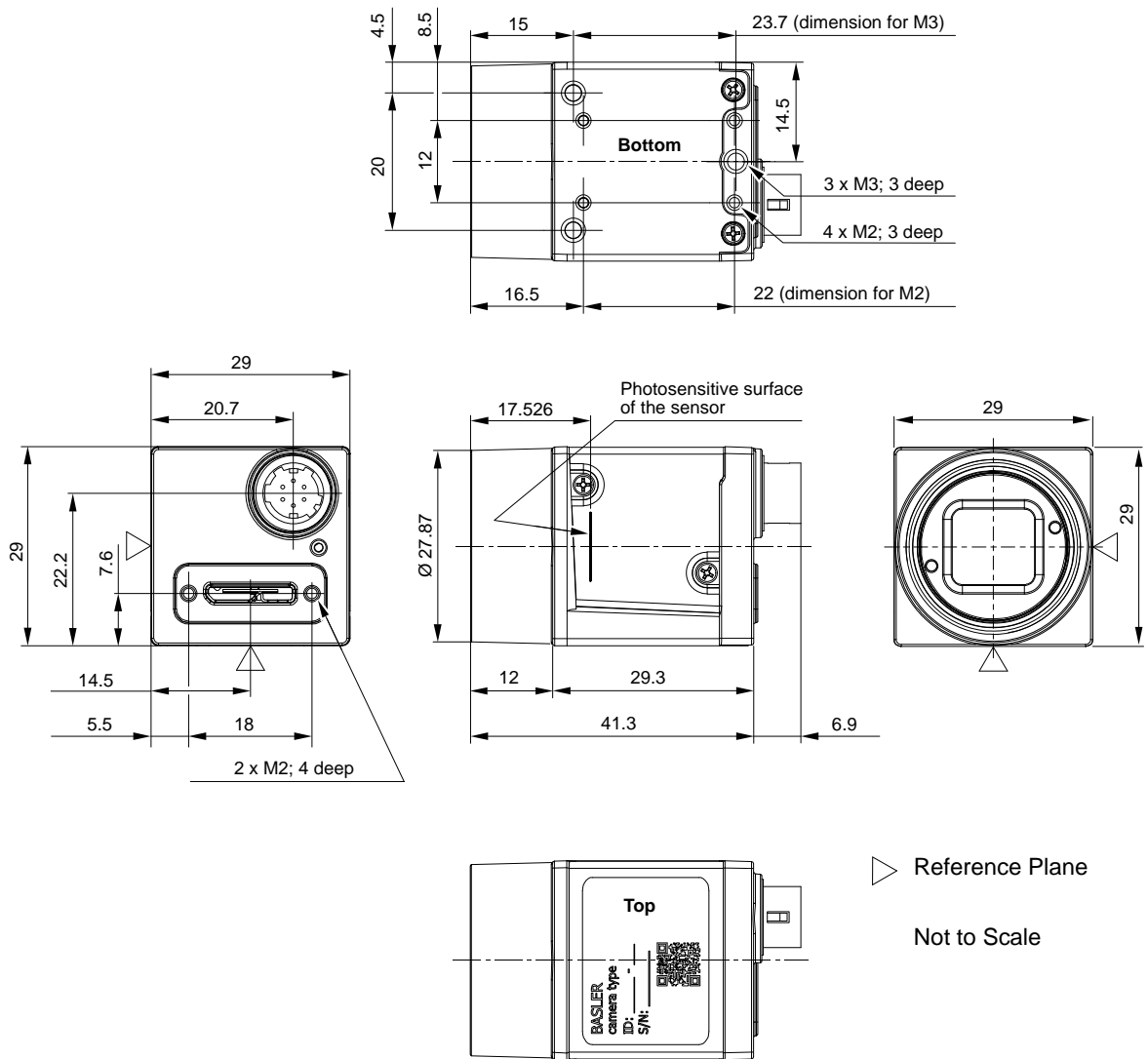
Fig. 25: Mechanical Dimensions (in mm) for Cameras with the C-mount
