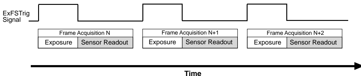
Fig. 65: Non-overlapped Exposure and Sensor Readout
