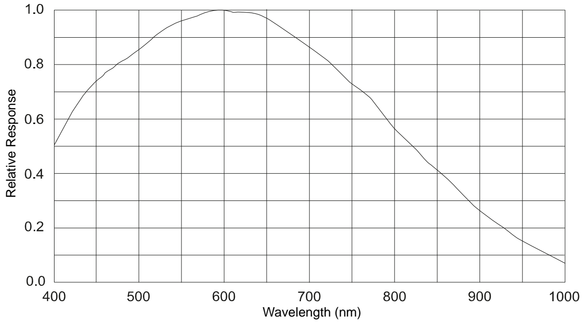
Fig. 10: acA2040-55um, acA2040-120um, acA2440-35um, and acA2440-75um (From Sensor Data Sheet)
