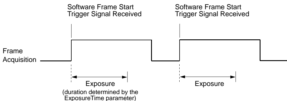
Fig. 54: Frame Acquisition with a Software Frame Start Trigger
