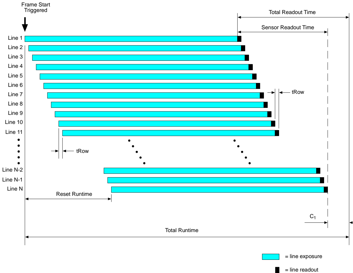
Fig. 61: Rolling Shutter in Rolling Mode
