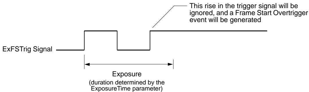
Fig. 56: Overtriggering with Timed Exposure
