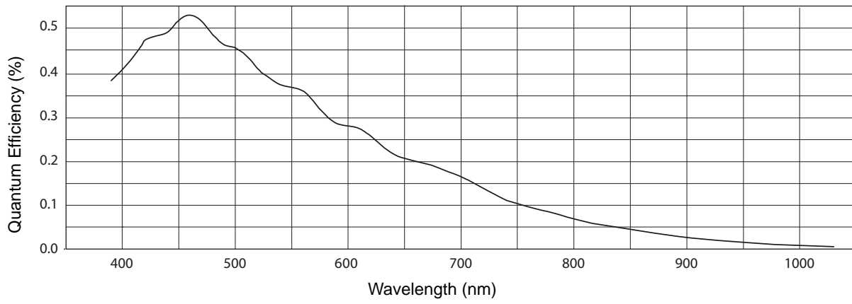
Fig. 12: acA3800-14um Spectral Response (From Sensor Data Sheet)
