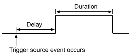
Fig. 50: Timer Signal
