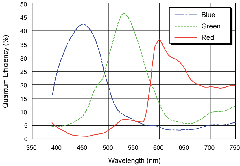
Fig. 22: acA2500-14uc Spectral Response (From Sensor Data Sheet)
