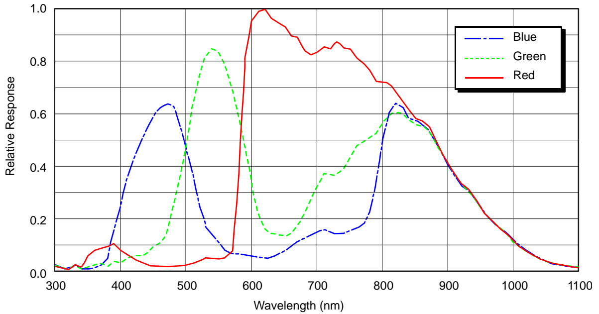
Fig. 17: acA640-750uc, acA800-510uc, acA1300-200uc, acA1920-150uc, and acA2500-60um, Spectral Response (From Sensor Data Sheet)
