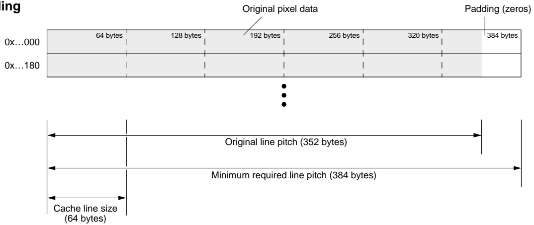
Fig. 114: Storage of Pixel Data from the First Two ROI Lines, Without and With Padding for 64-byte Alignment
