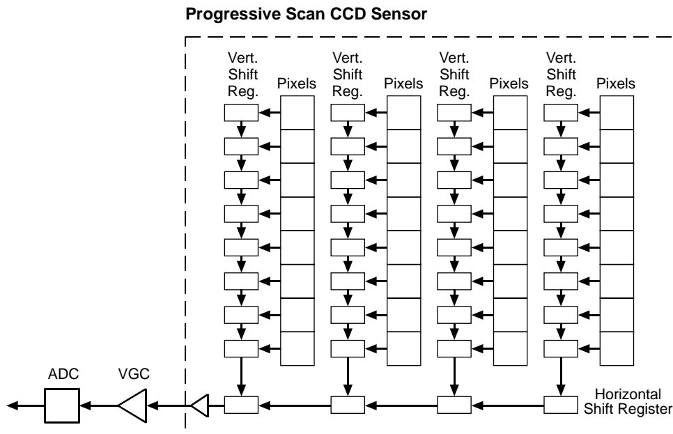
Fig. 33: CCD Sensor Architecture - Progressive Scan Sensors
