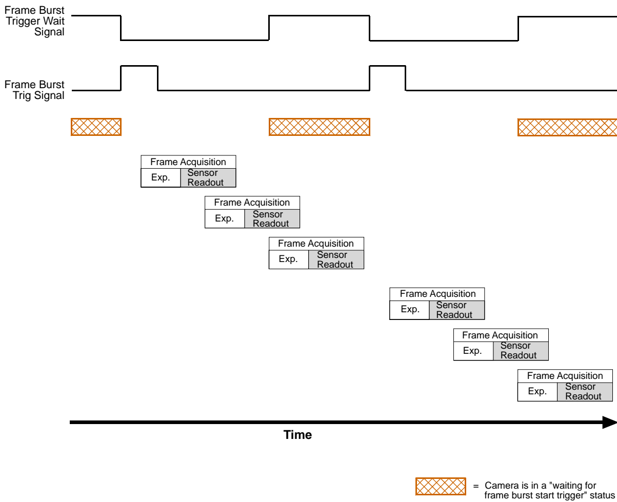
Fig. 74: Frame Burst Trigger Wait Signal
