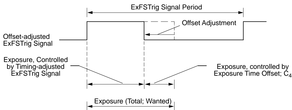
Fig. 59: Trigger Width Exposure with Adjusted Rising Edge Triggering; (Exposure Start Delay Is Omitted)
