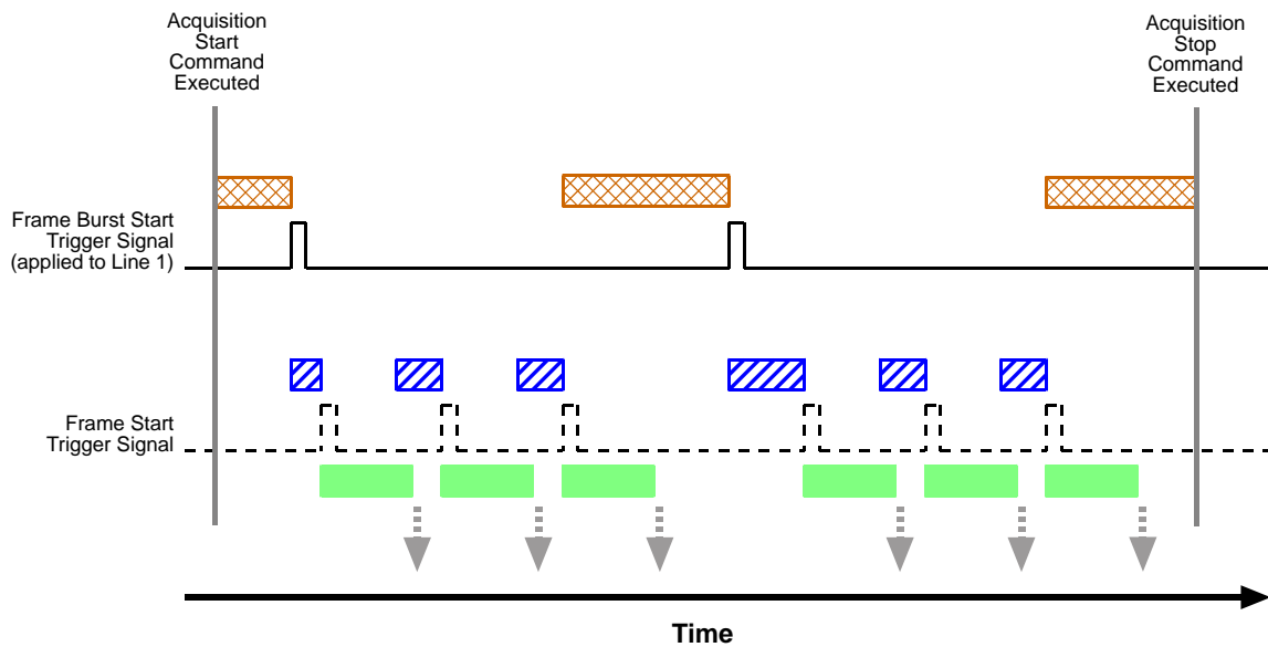
Fig. 82: Use Case 3 - Frame Burst Start Trigger On and Frame Start Trigger Off
