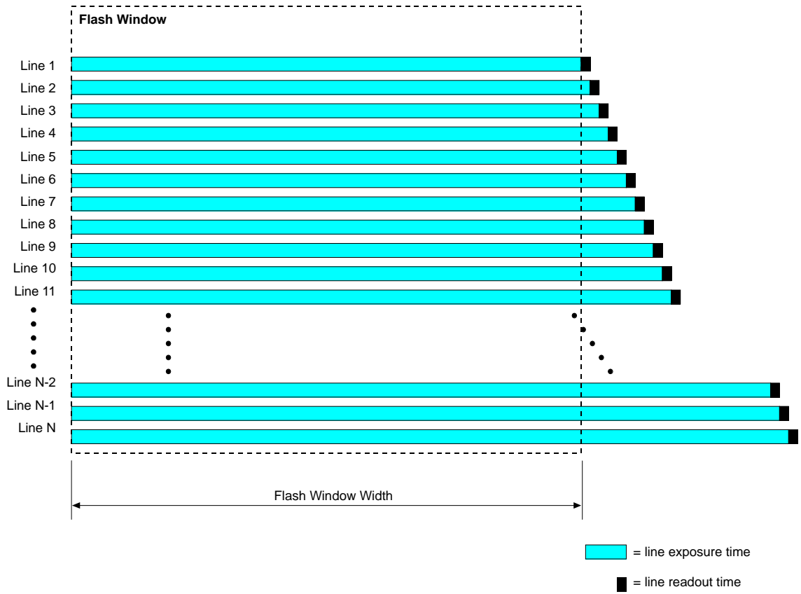
Fig. 64: Flash Window for Rolling Shutter in Global Reset Release Mode
