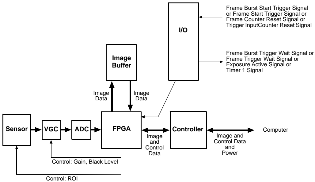
Fig. 34: Camera Block Diagram
