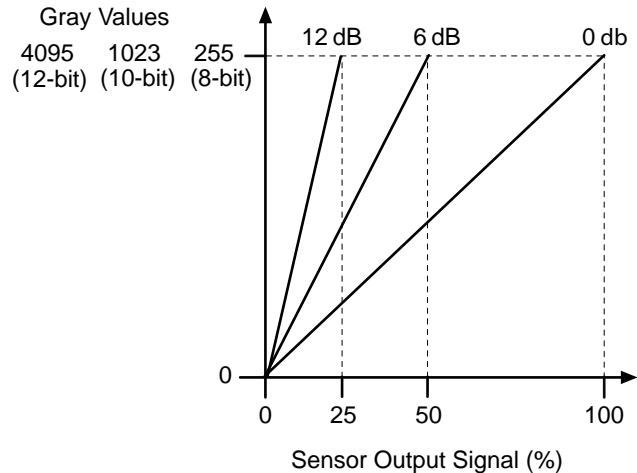
Fig. 84: Gain in dB, Shown for 8 bit, 10 bit, and 12 bit Output
