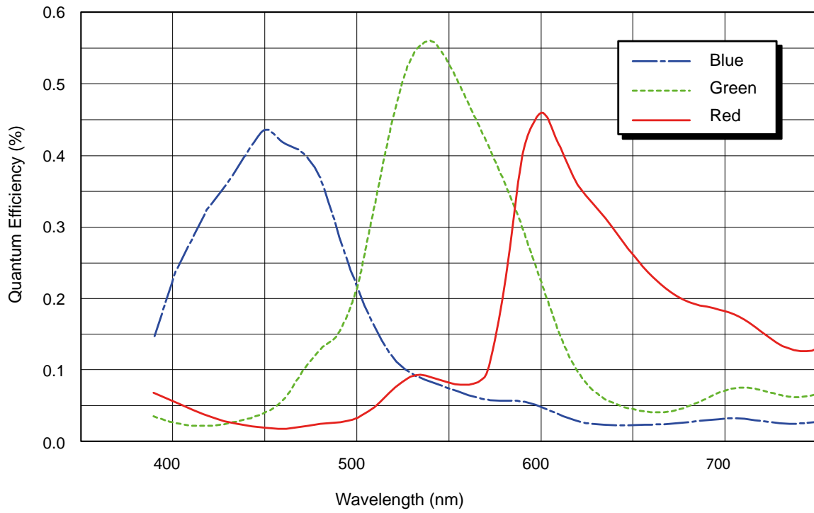
Fig. 24: acA4600-10uc Spectral Response (From Sensor Data Sheet)
