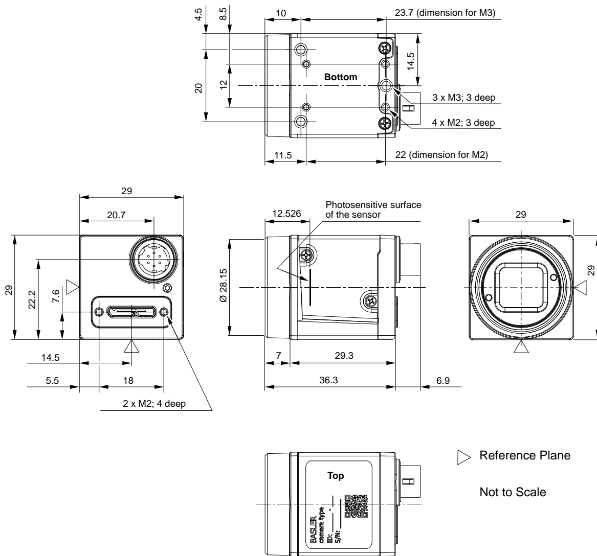
Fig. 26: Mechanical Dimensions (in mm) for Cameras with the CS-mount
