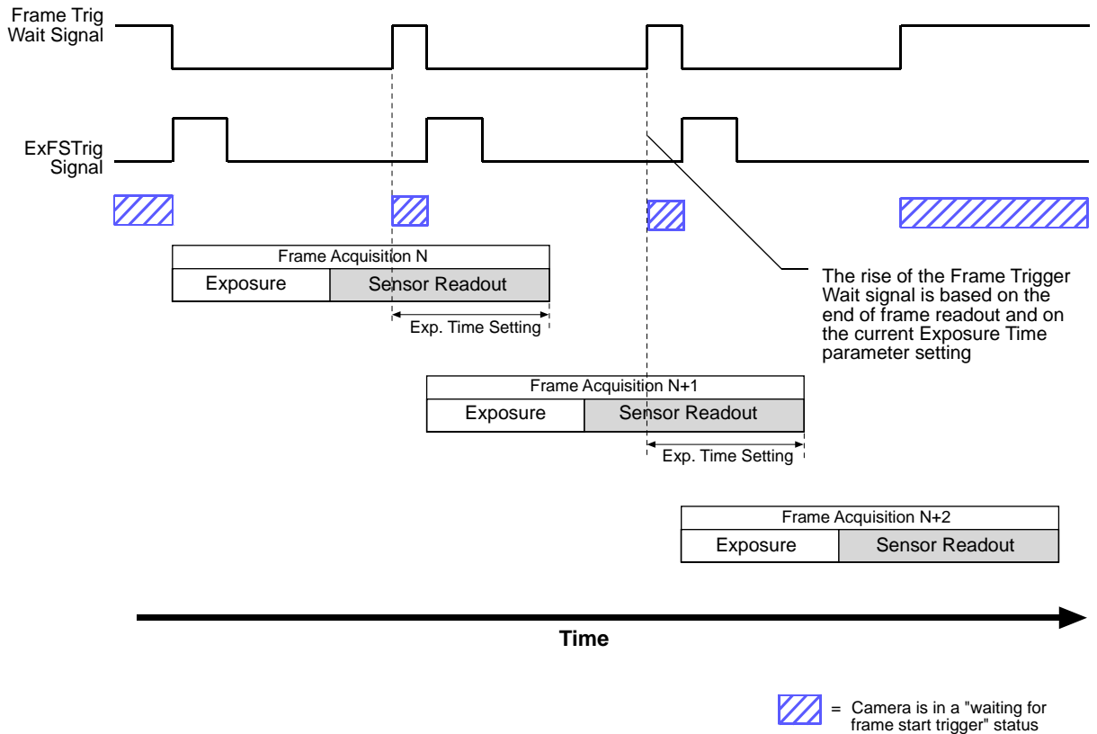
Fig. 76: Frame Trigger Wait Signal with the Timed Exposure Mode
