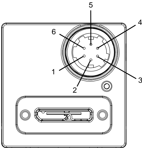
Fig. 38: Pin Numbering for the 6-pin Connector
