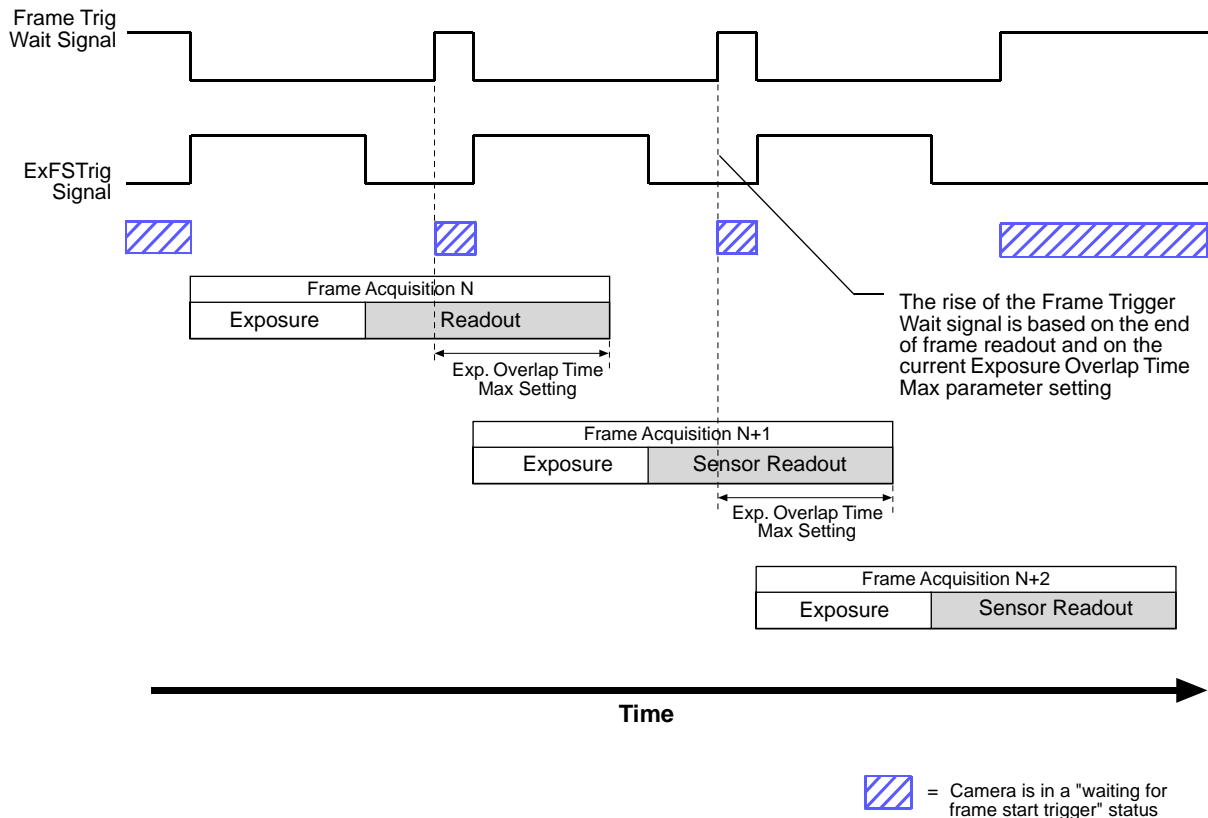
Fig. 77: Frame Trigger Wait Signal with the Trigger Width Exposure Mode
