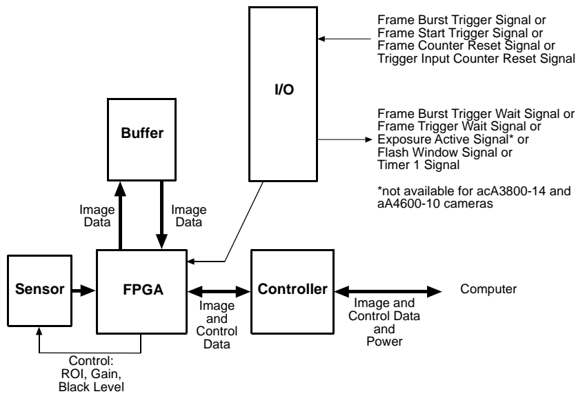
Fig. 36: Camera Block Diagram
