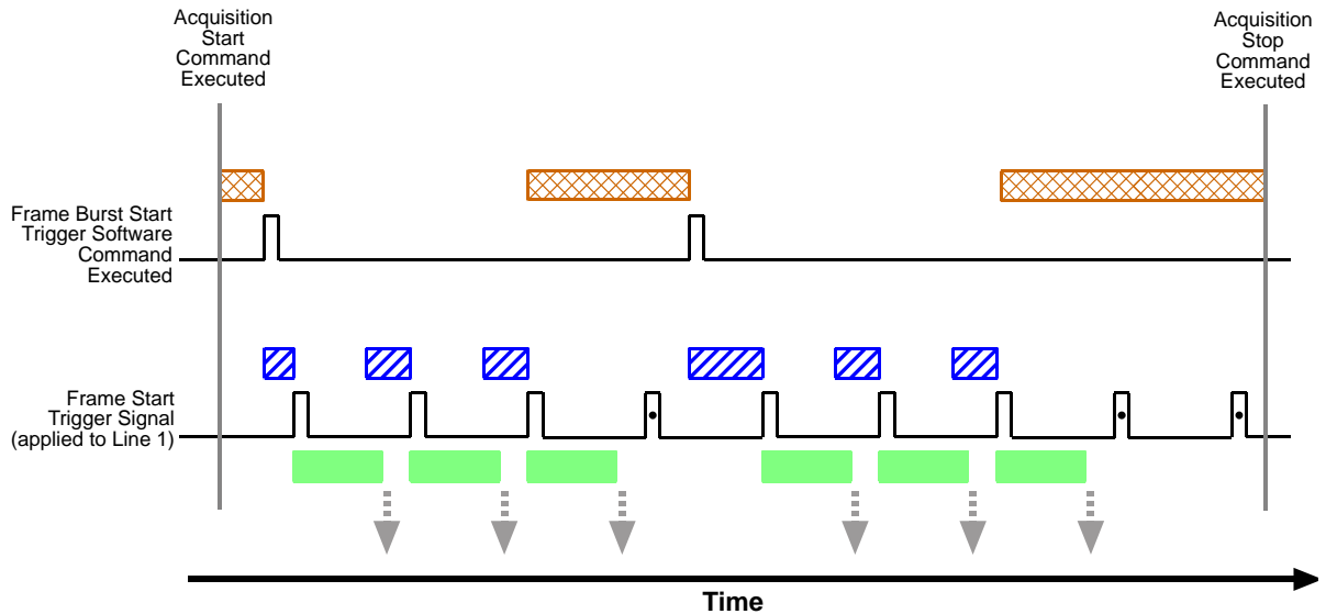
Fig. 83: Use Case 4 - Frame Burst Start Trigger On and Frame Start Trigger On
