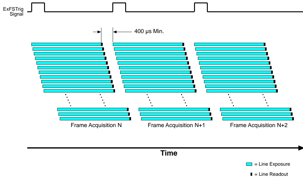
Fig. 70: Acquisition Overlap Guideline
