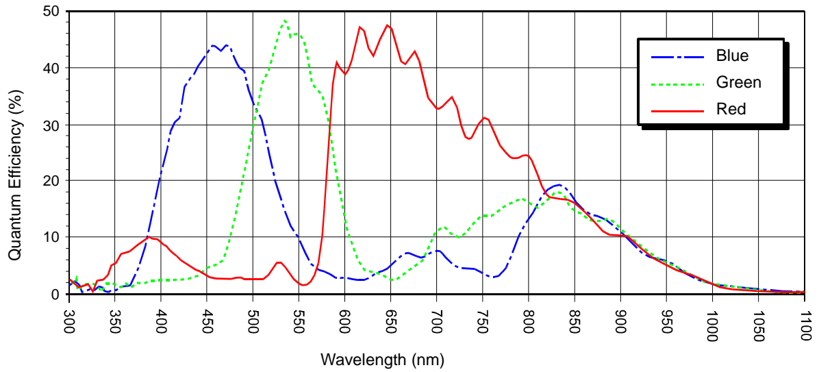
Fig. 20: acA2000-165uc, acA2040-90uc Spectral Response (From Sensor Data Sheet)
