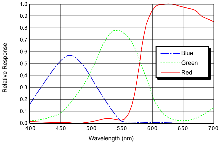
Fig. 14: acA640-120uc Spectral Response (From Sensor Data Sheet)
