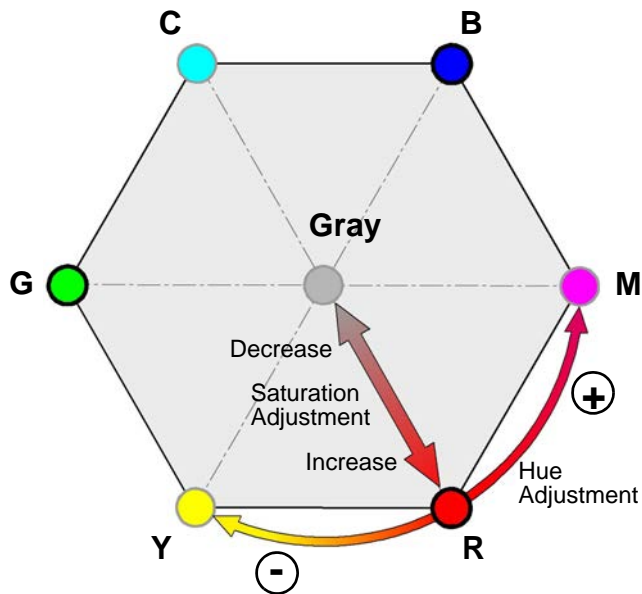
Fig. 108: Hue and Saturation Adjustment In the Color Hexagon. Adjustments Are Indicated for Red as an Example
