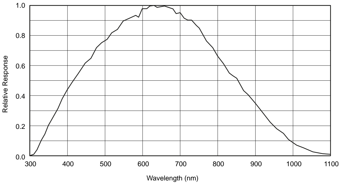
Fig. 5: acA640-750um, acA800-510um, acA1300-200um, acA1920-150um, and acA2500-60um, Spectral Response (From Sensor Data Sheet)
