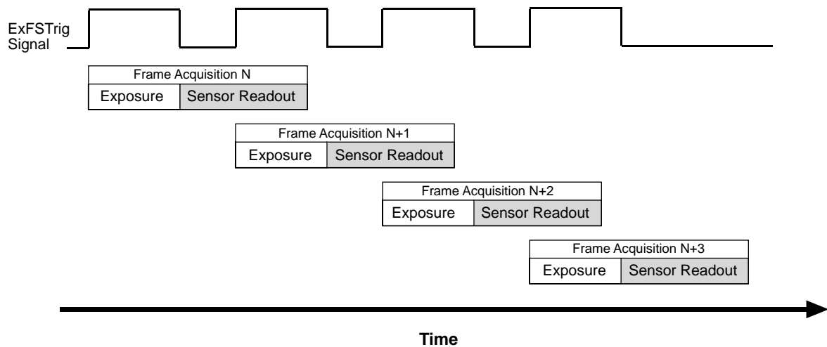
Fig. 66: Overlapped Exposure and Sensor Readout
