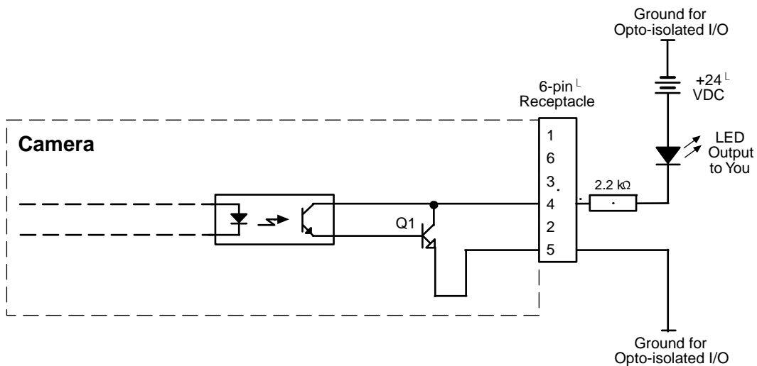
Fig. 41: Opto-isolated Output Line Schematic with a Typical LED Output Signal at +24 VDC for the External Circuit (Simplified)
