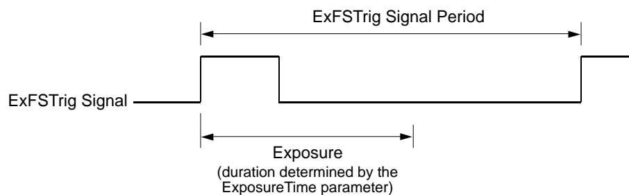
Fig. 55: Timed Exposure with Rising Edge Triggering
