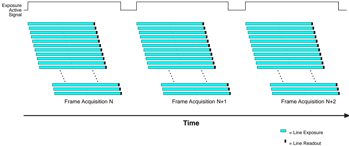
Fig. 72: Exposure Active Signal on Cameras Operating in Rolling Mode
