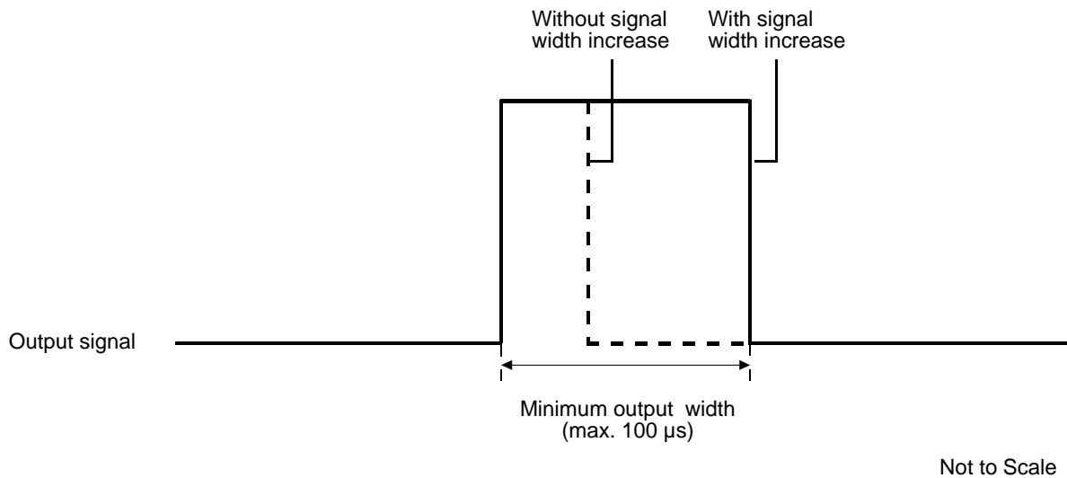
Fig. 48: Increasing the Signal Width of an Output Signal
