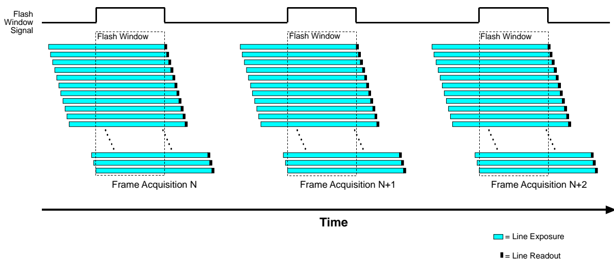
Fig. 73: Flash Window Signal on Cameras Operating in Rolling Mode
