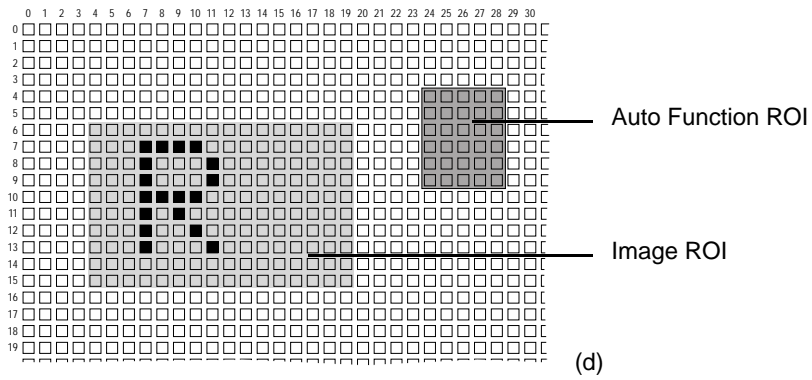
Fig. 110: Various Degrees of Overlap Between the Auto Function ROI and the Image ROI
