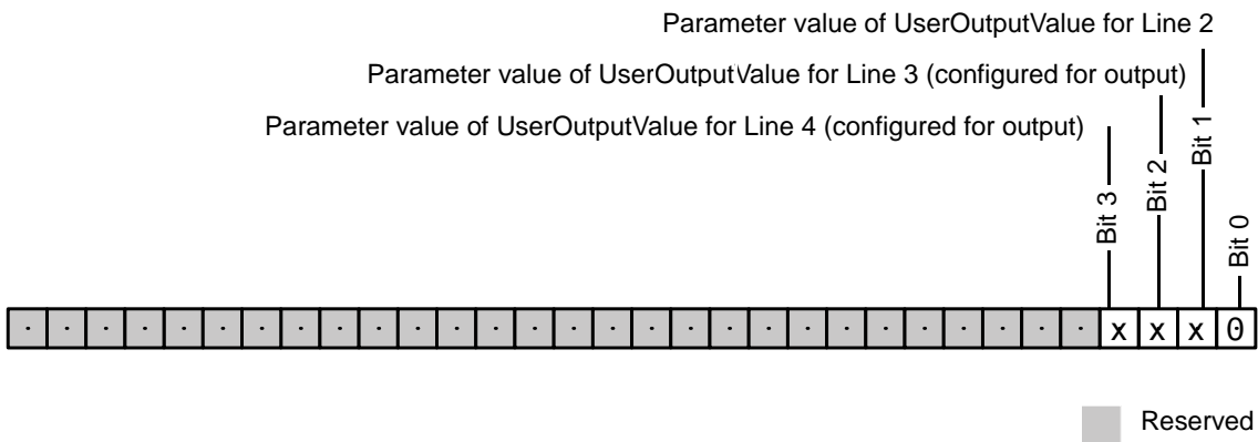
Fig. 49: Bit Field of the UserOutputValueAll Parameter: Bit Numbers and Assignment of Output Lines
