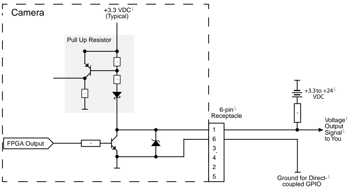
Fig. 44: Direct-coupled GPIO Line Schematic with the GPIO Line Set as an Output and with a Typical Voltage Output Circuit (Illustration for Pin 1 as an Example; Simplified)
