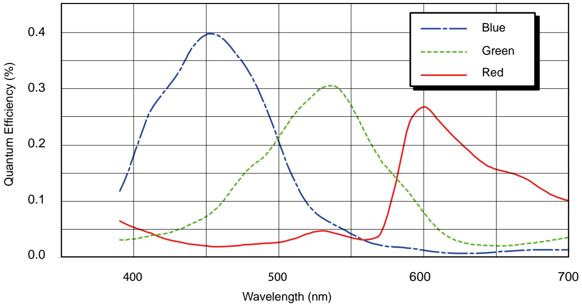
Fig. 23: acA3800-14uc Spectral Response (From Sensor Data Sheet)
