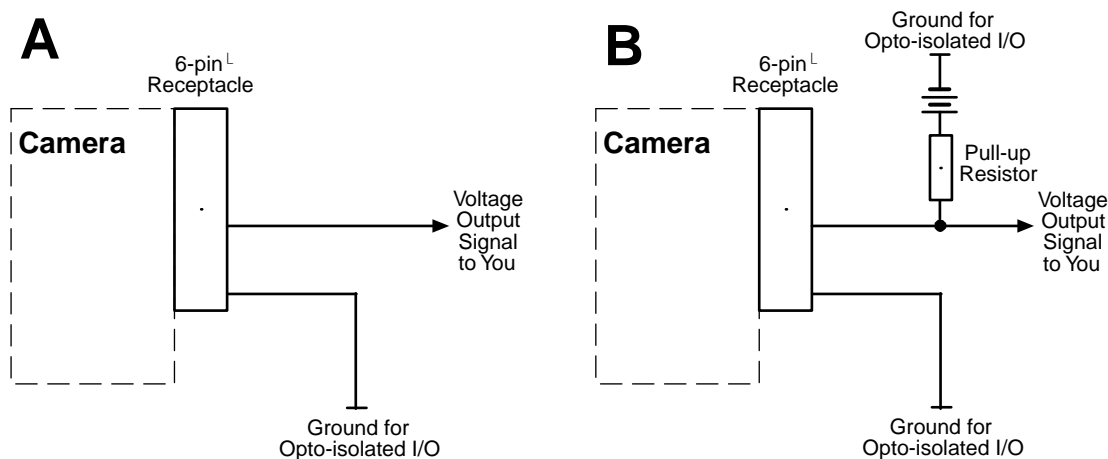
Fig. 51: Use of an External Pull-up Resistor With an Output Line: A : No External Pull-up Resistor Connected, B : External Pull-up Resistor Connected
