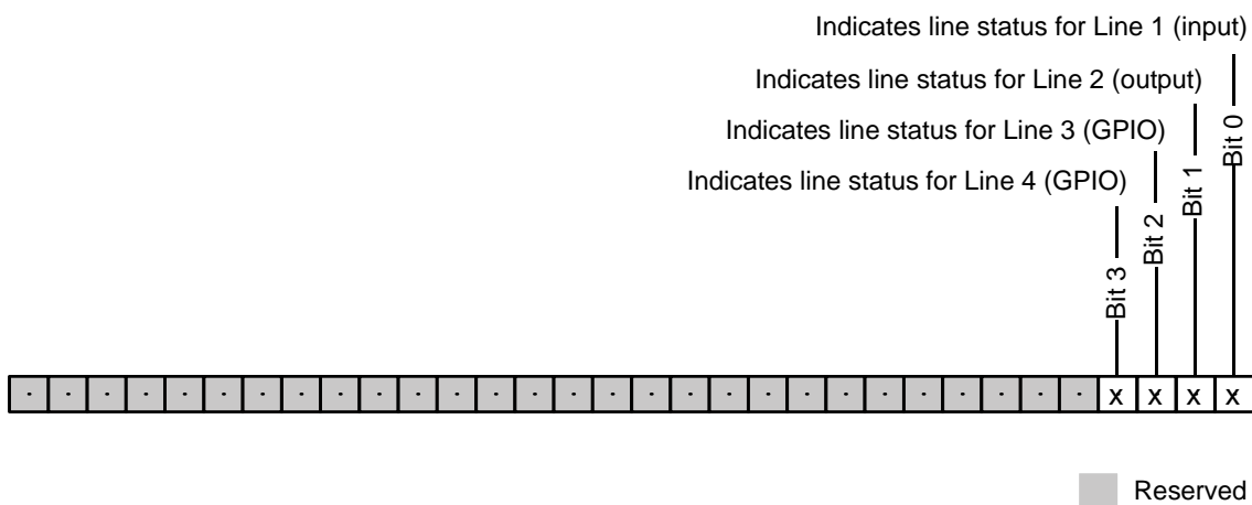
Fig. 52: Bit Field of the LineStatusAll Parameter: Bit numbers and Assignment of I/O Lines
