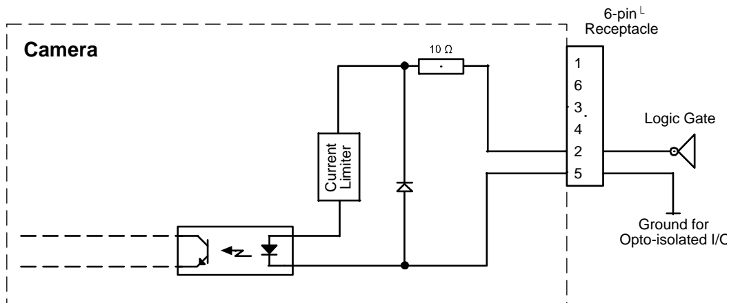
Fig. 39: Opto-isolated Input Line Schematic with a Typical External Circuit (Simplified)
