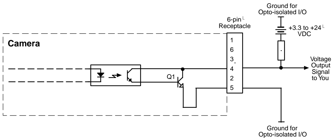
Fig. 40: Opto-isolated Output Line Schematic with a Typical Voltage Output Circuit (Simplified)
