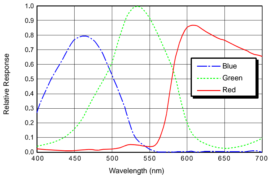
Fig. 13: acA640-90uc Spectral Response (From Sensor Data Sheet)
