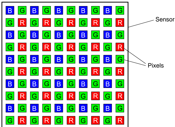
Fig. 106: Bayer Filter Pattern With "BG" Physical Alignment as an Example
