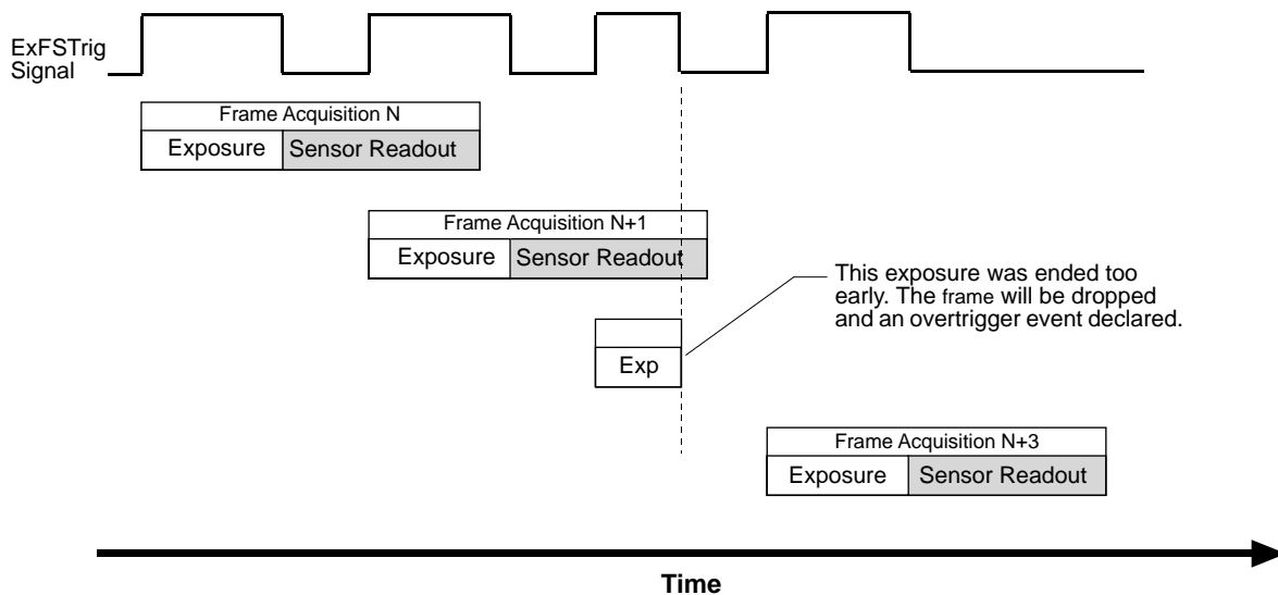
Fig. 67: Overtriggering Caused by an Early End of Exposure
