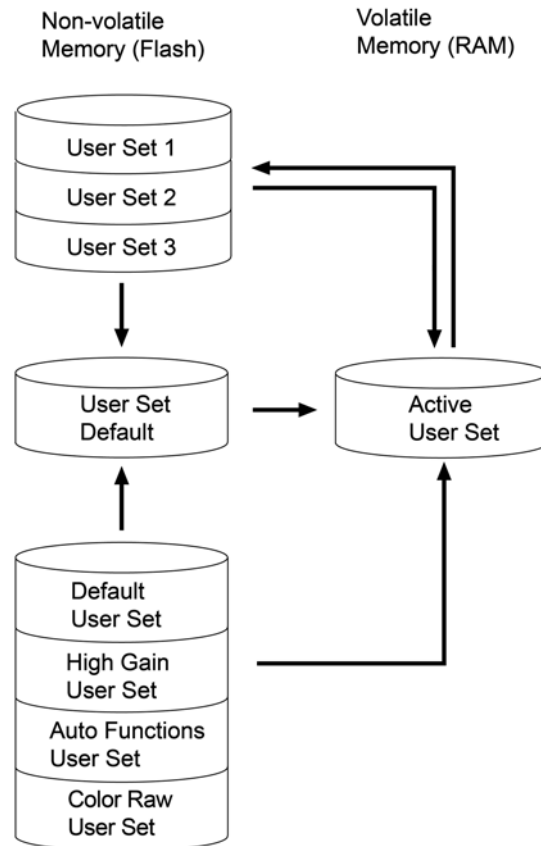
Fig. 113: User Sets
