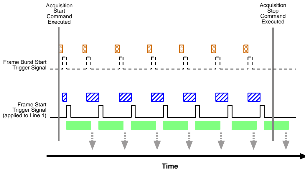
Fig. 81: Use Case 2 - Frame Burst Start Trigger Off and Frame Start Trigger On
