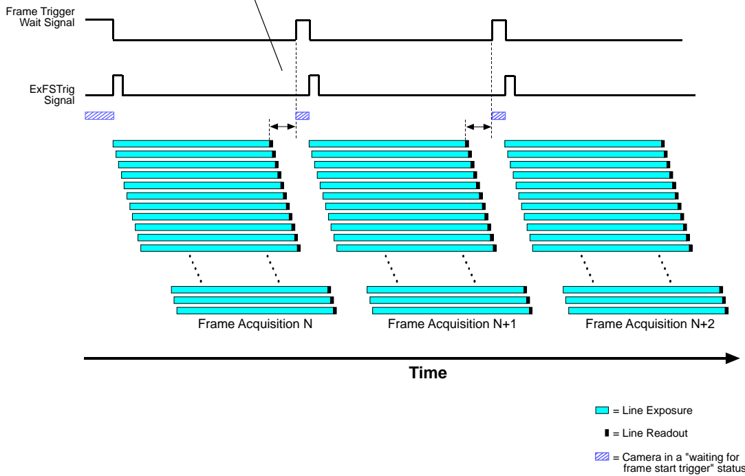
Fig. 78: Frame Trigger Wait Signal on a Rolling Shutter Camera
