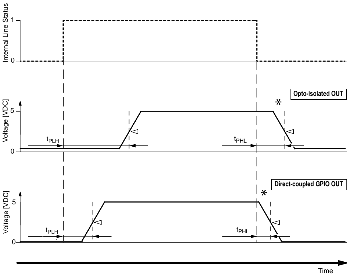
Fig. 46: Internal Line Status and Associated Output Signals with Propagation Delays for Opto-isolated Output and Direct-coupled GPIO Outputs (Line Inverters Disabled)
