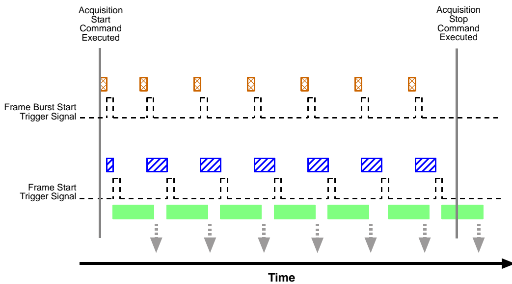
Fig. 80: Use Case 1 - Frame Burst Start Trigger Off and Frame Start Trigger Off
