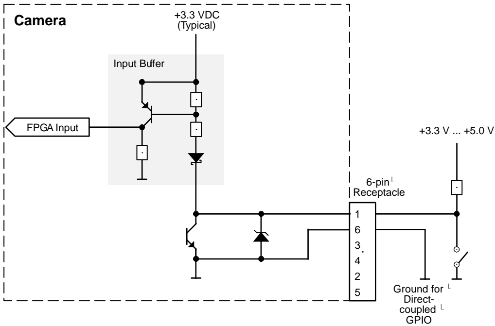
Fig. 43: Direct-coupled GPIO Line Schematic with the GPIO Line Set as an Input and with a Typical External Circuit (Illustration for Pin 1 as an Example; Simplified)
