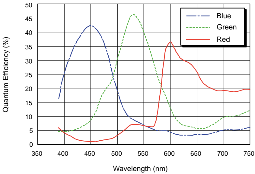
Fig. 18: acA1920-25uc Spectral Response (From Sensor Data Sheet)
