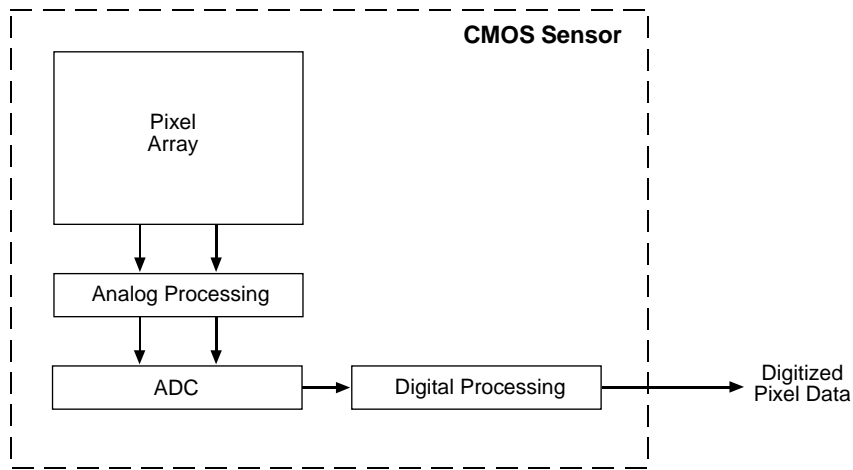
Fig. 35: CMOS Sensor Architecture
