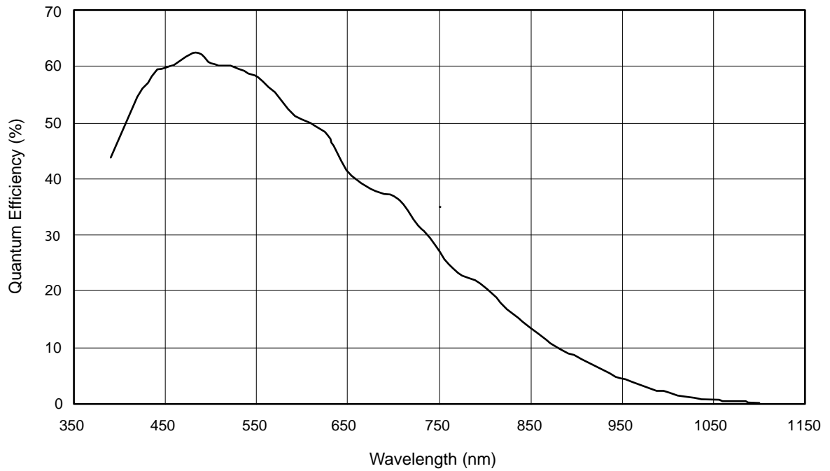
Fig. 11: acA2500-14um Spectral Response (From Sensor Data Sheet)
