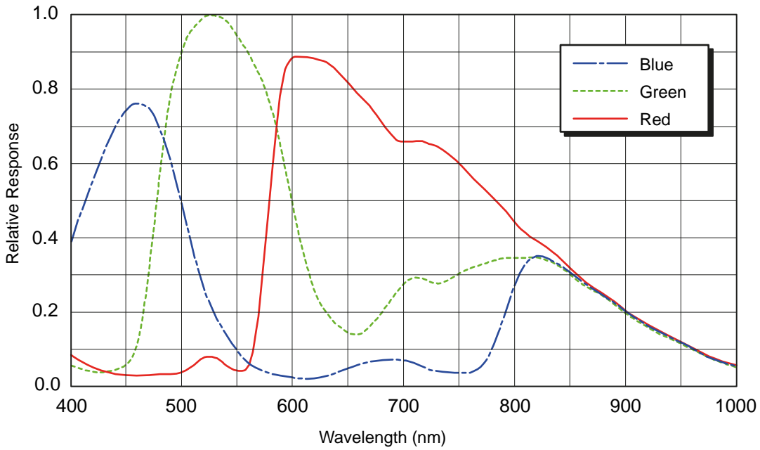
Fig. 19: acA1920-40uc and acA1920-155uc (From Sensor Data Sheet)
