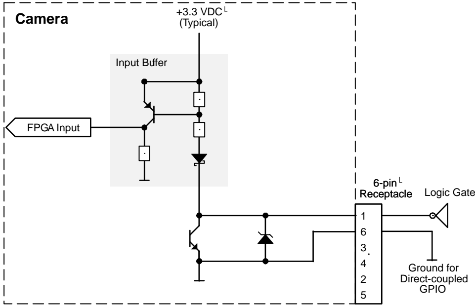
Fig. 42: Direct-coupled GPIO Line Schematic with the GPIO Line Set as an Input and with a Typical External Circuit Using a Logic Gate (Illustration for Pin 1 as an Example; Simplified)
