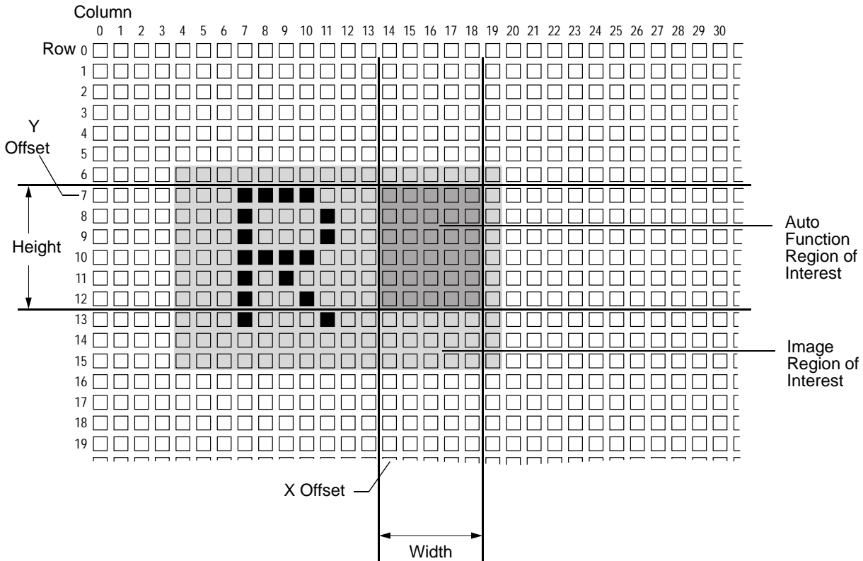
Fig. 109: Auto Function Region of Interest and Image Region of Interest
